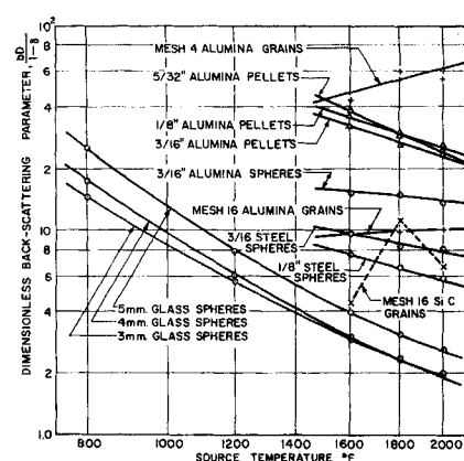
Fig. 7. Back scattering parameter for packed beds.
